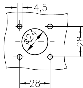
mounting dimension
